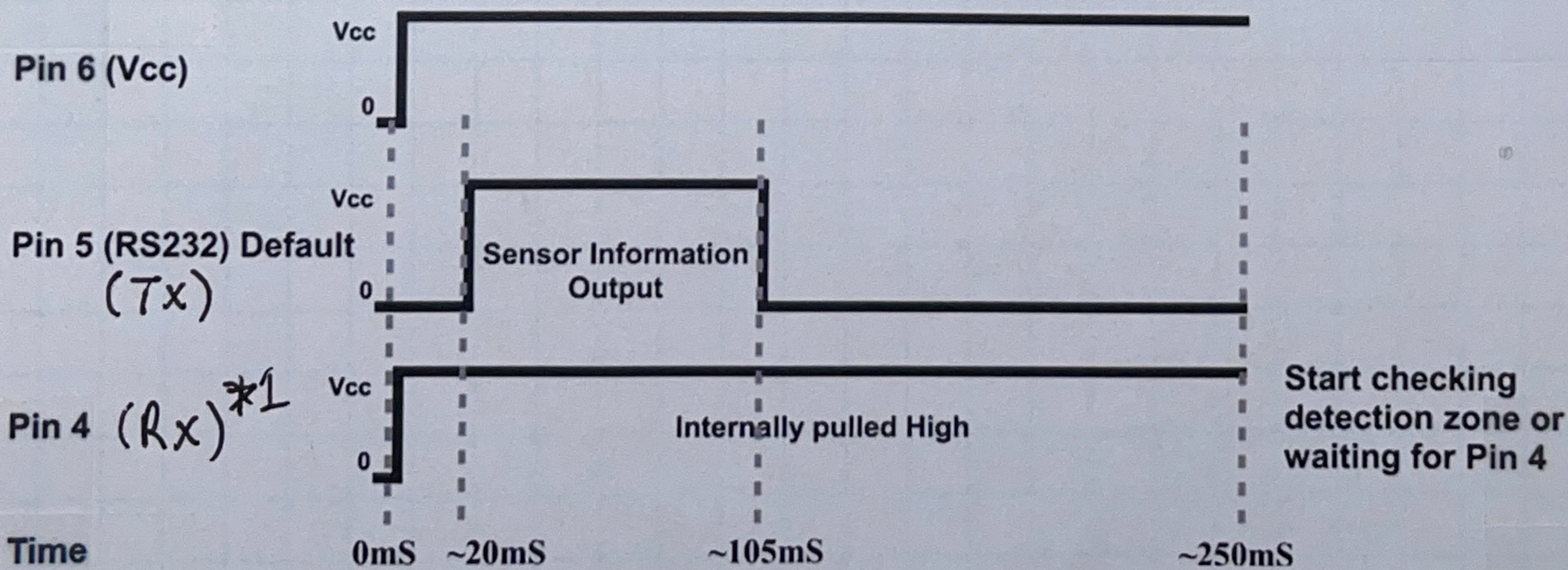
Power-Up Timing Diagram
